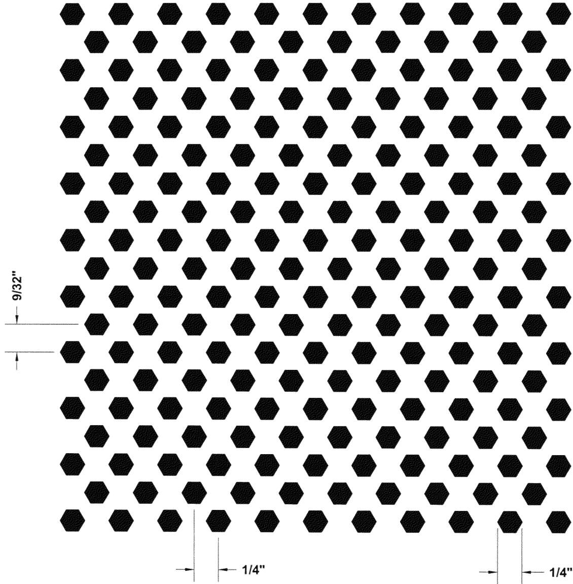
PERFORATION No. (SP-2) 1/4" HEXAGONAL HOLES @ 1/4" x 9/32" STAGGERED CENTERS (20% OPEN)
