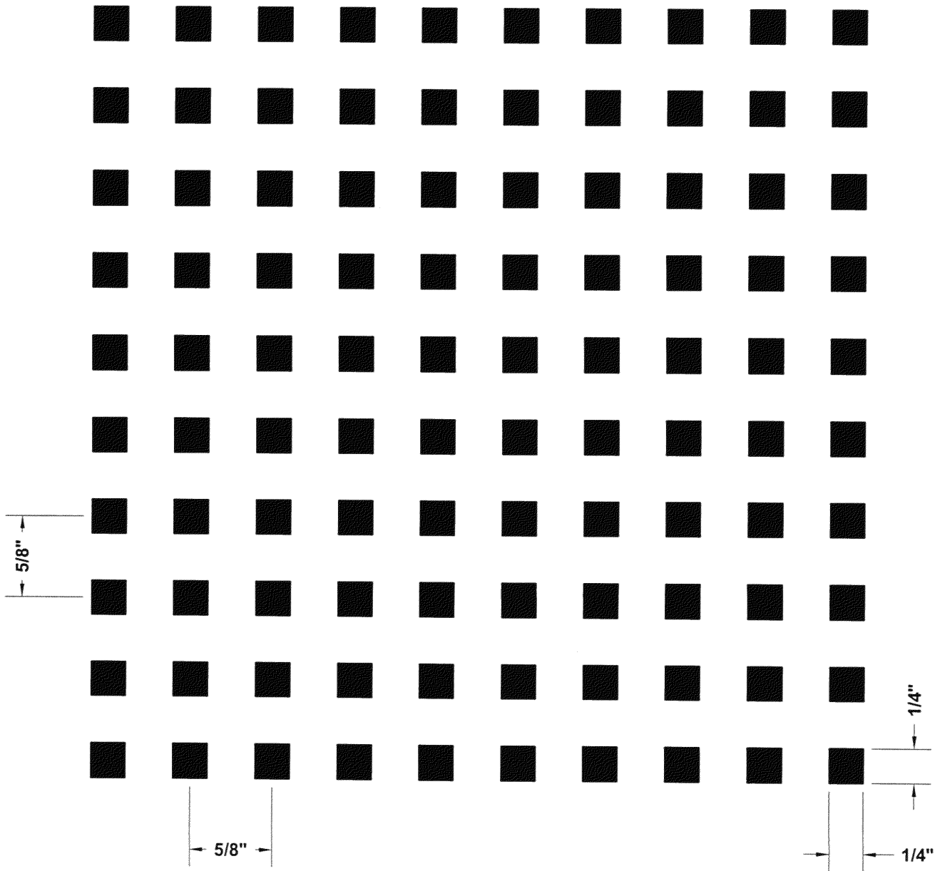
PERFORATION No. (S-3) 1/4" SQUARE HOLES @ 5/8" STRAIGHT CENTERS (17% OPEN)
