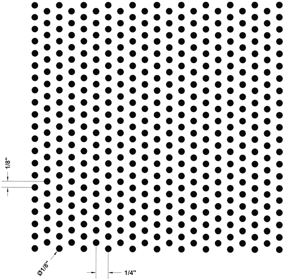
PERFORATION No. (R-20) 1/8" DIA. HOLES @ 1/4" x 1/8" STAGGERED CENTERS (23% OPEN)
