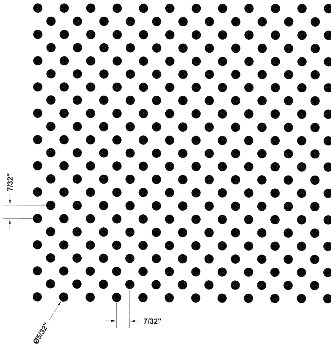
PERFORATION No. (R-18) 5/32" DIA. HOLES @ 7/32" DIAGONAL CENTERS (18% OPEN)
