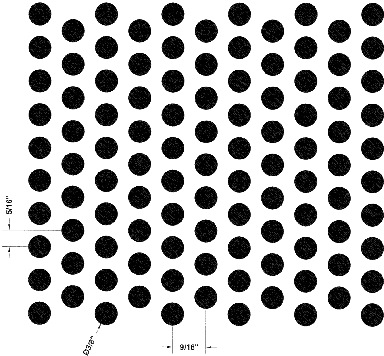
PERFORATION No. (R-16) 3/8" DIA. HOLES @ 9/16" x 5/16" STAGGERED CENTERS (18% OPEN)
