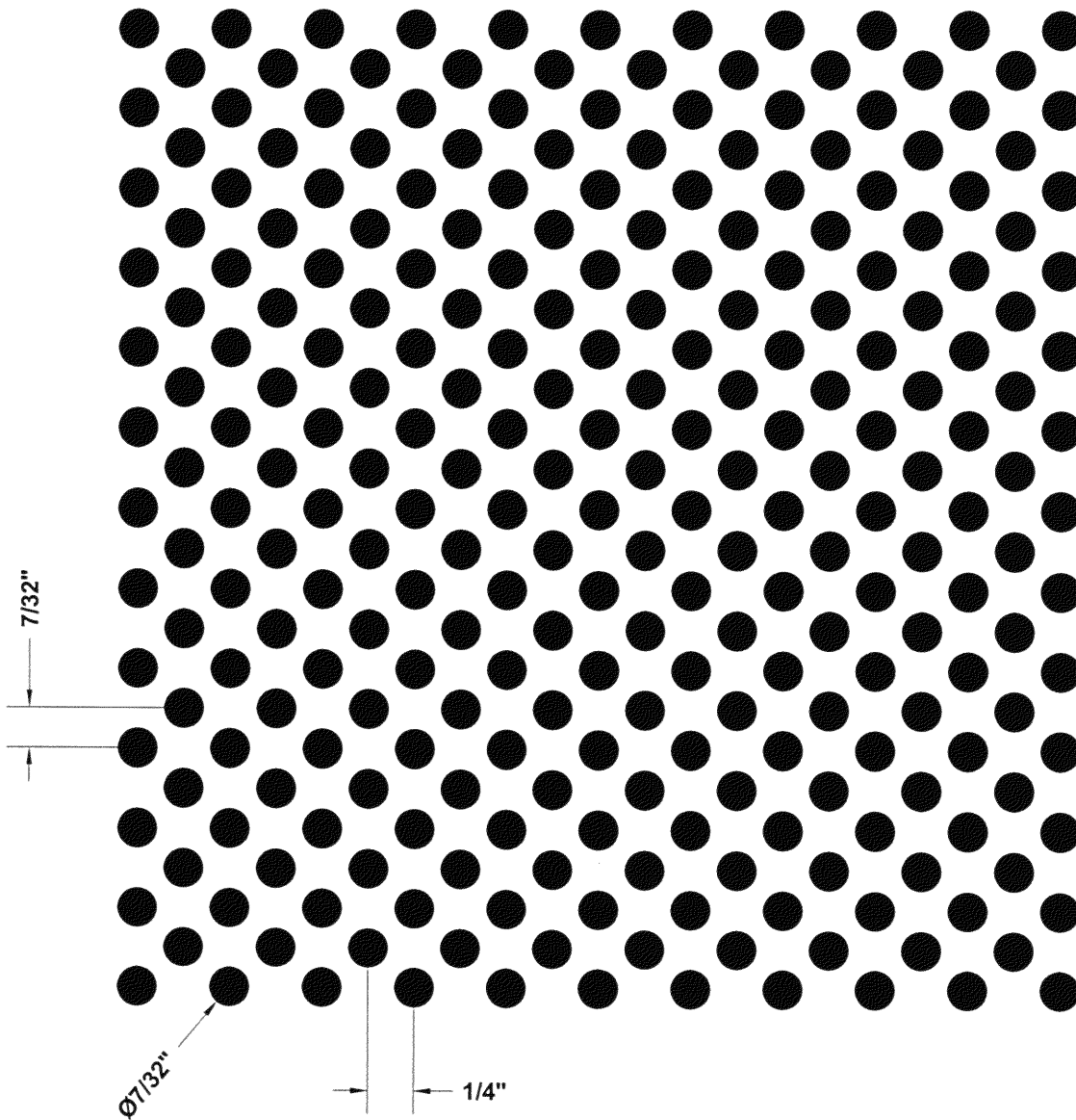
PERFORATION No. (R-15) 7/32" DIA. HOLES @ 1/4" x 7/32" STAGGERED CENTERS (18% OPEN)
