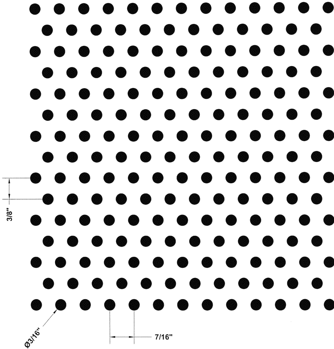
PERFORATION No. (R-14) 3/16" DIA. HOLES @ 7/16" x 3/8" STAGGERED CENTERS (17% OPEN)
