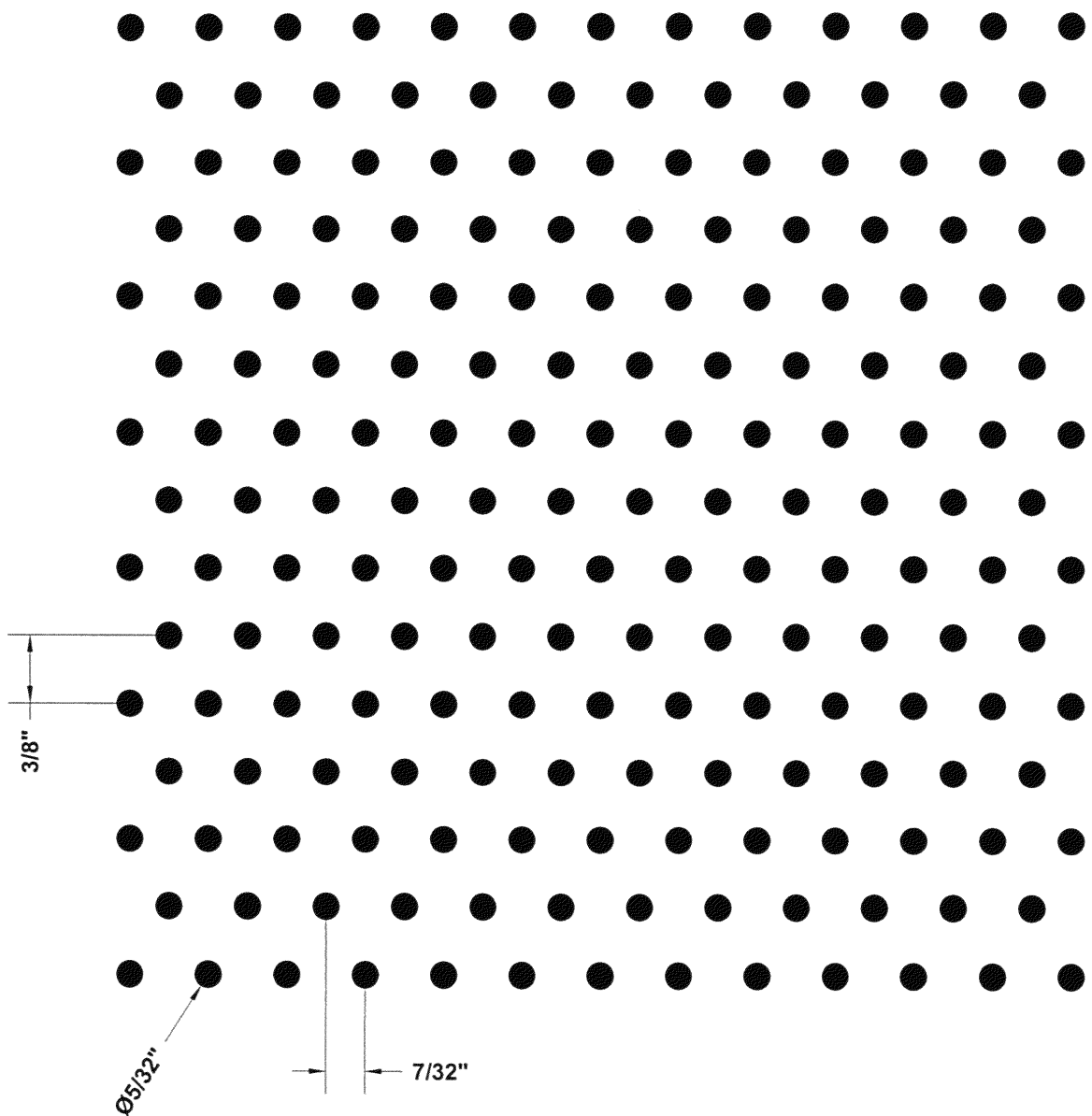
PERFORATION No. (R-12) 5/32" DIA. HOLES @ 7/32" x 3/8" STAGGERED CENTERS (12% OPEN)
