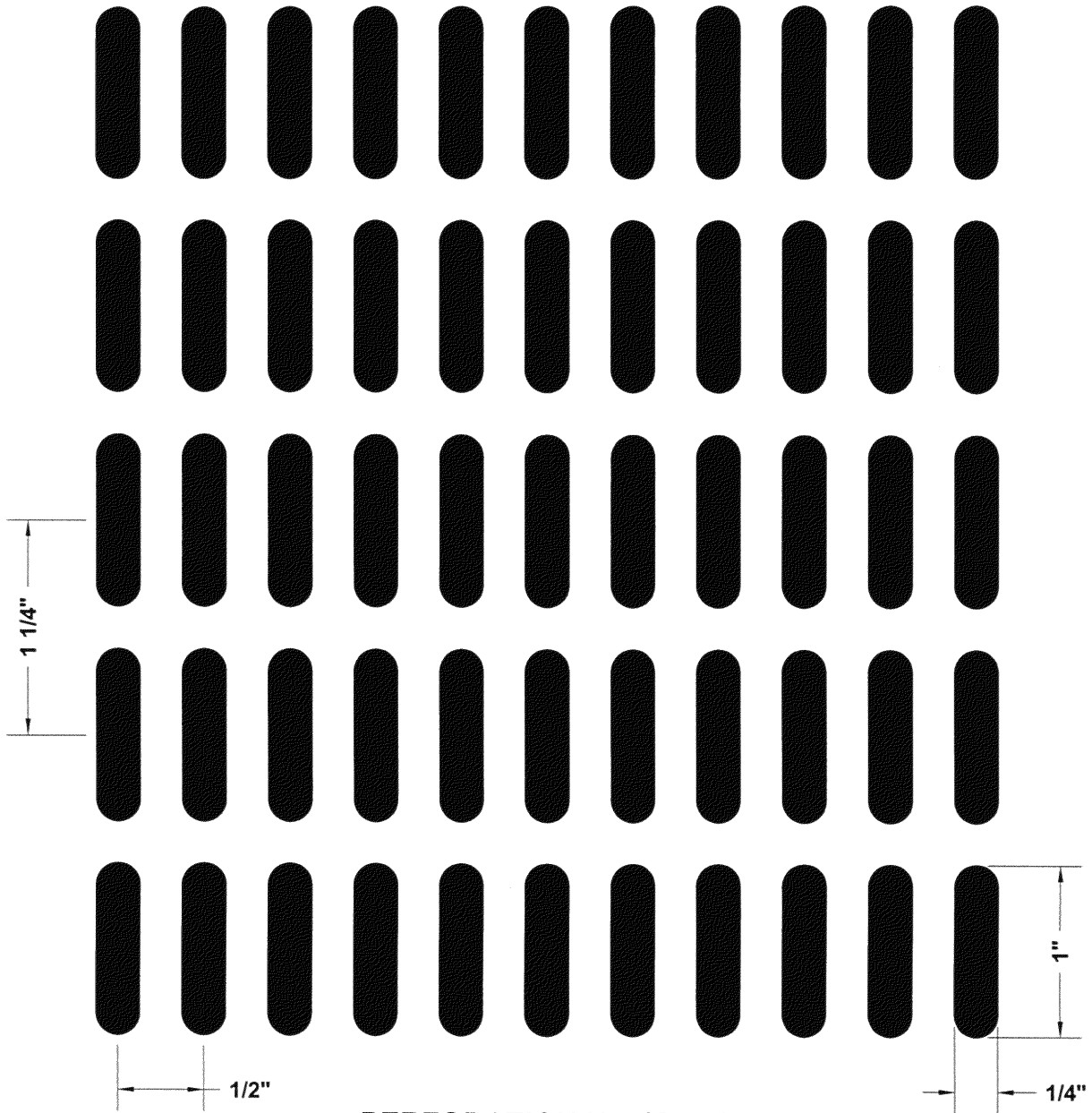
PERFORATION No. (OB-3) 1/4" x 1" OBROUND HOLES @ 1/2" x 1 1/4" STRAIGHT CENTERS (38% OPEN)
