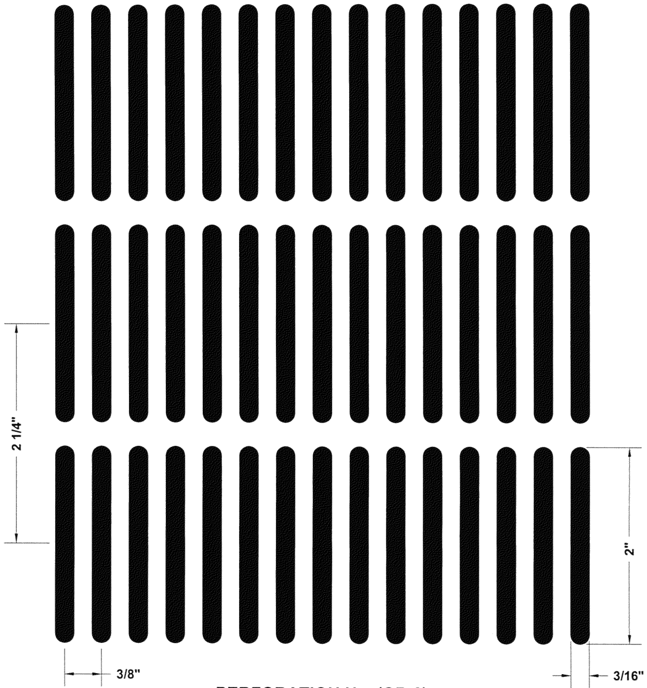
PERFORATION No. (OB-2) 3/16" x 2" OBOUNDR HOLES @ 3/8" x 2 1/4" STRAIGHT CENTERS (43% OPEN)
