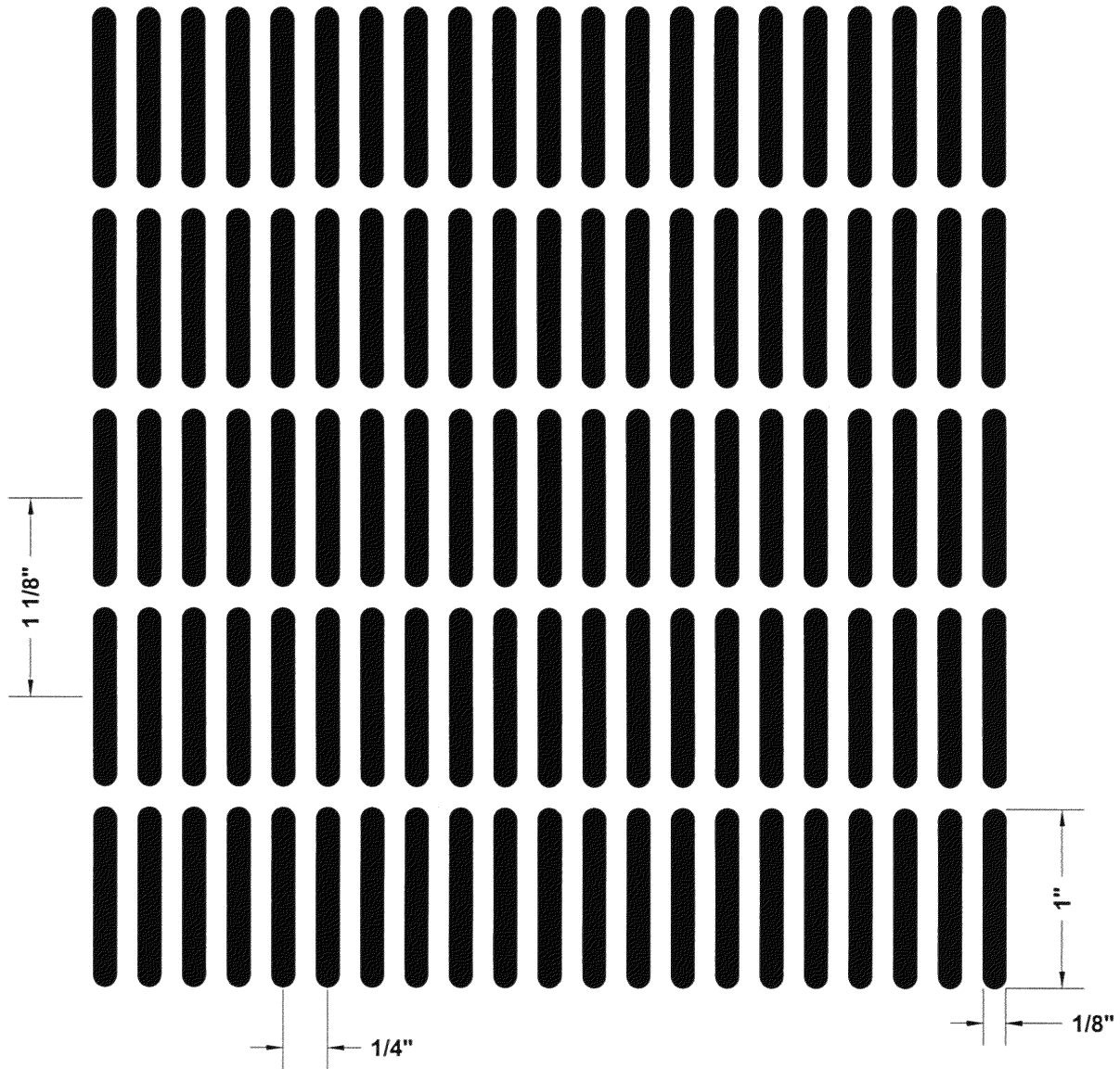
PERFORATION No. (OB-1) 1/8" x 1" OBROUND HOLES @ 1/4" x 1 1/8" STRAIGHT CENTERS (43% OPEN)
